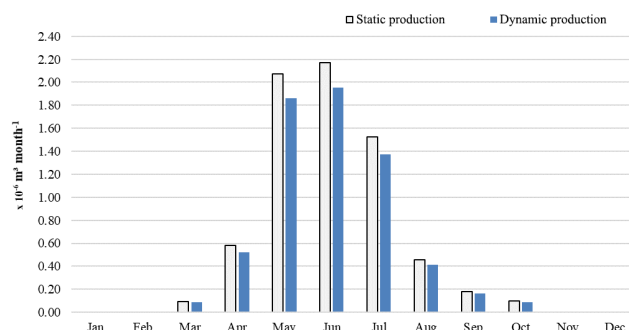
Figure 7. Monthly groundwater use by static and dynamic production of phosphate slurries transported by pipeline.
