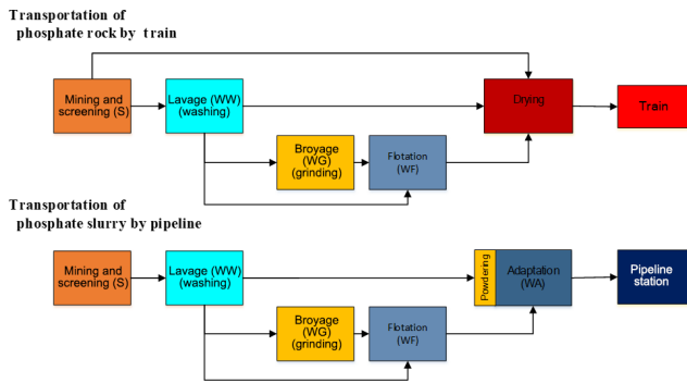
Figure 3. The functional processes and flows of products in Khouribga (mining area) by transportation method.
