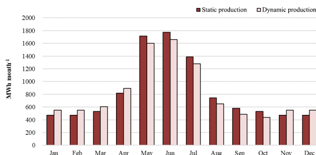
Figure 8. Monthly electricity consumption for supplying water by static and dynamic production of phosphate slurries transported by pipeline.
