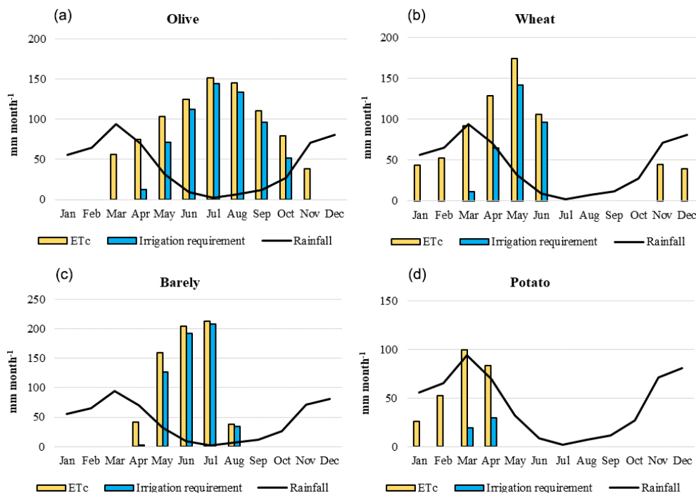
Figure 5. Monthly irrigation water requirement and rainfall in Khouribga.
