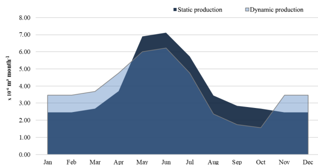
Figure 6. Monthly water supply from Ait Messaoud Dam.
