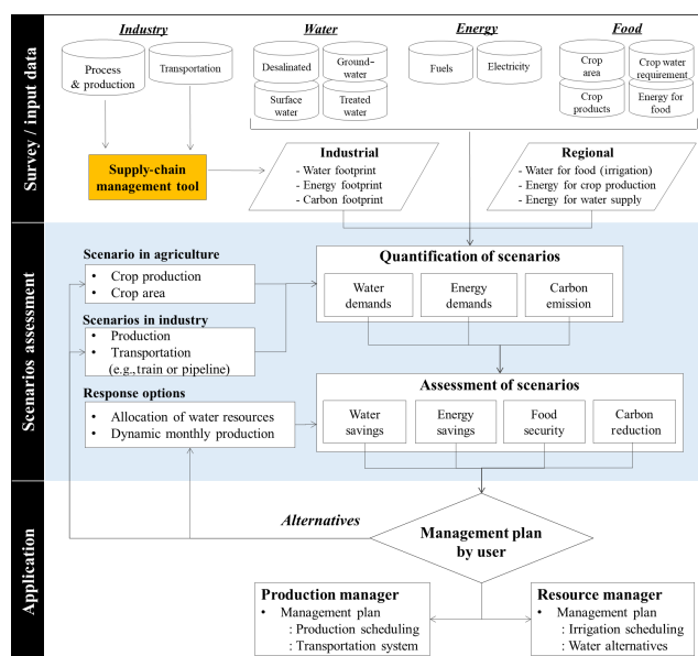
Figure 2. Assessment of holistic impacts of various scenarios relating to the phosphate industry, agriculture, and resource management using WEF-P Tool.
