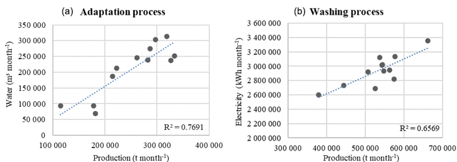
Figure 4. Water and energy footprints in MEA based on the BAU database.
